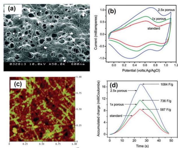
Fig. 8 (a) SEM image of an etched porous SWNT film, (b) cyclic voltammograms for \text{RuO}_2/\text{SWNT} electrodes of standard, 1\times , and 2.5\times underlying SWNT film porosity at a scan rate of 50 \text{ mV s}^{-1} in 1 \text{ M H}_2\text{SO}_4 , (c) AFM image of \text{RuO}_2 electrodeposited onto a standard dense SWNT film, (d) integrated current vs. time plots for each \text{RuO}_2/\text{SWNT} electrode in cycling in the voltage range of 0\text{--}1.2 \text{ V vs. Ag/AgCl} reference electrode. Reproduced with permission from ref. 173. Copyright 2009 American Chemical Society.
