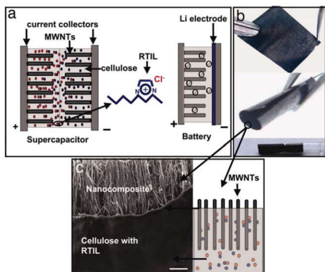
Fig. 7 Fabrication of self-supported CNT composite paper units for supercapacitors and batteries. (a) Schematic of the supercapacitor and battery assembled using nanocomposite film units. The nanocomposite unit comprises a room temperature ionic liquid and MWNT embedded inside cellulose paper. A thin extra layer of cellulose covers the top of the MWNT array. A Ti/Au thin film deposited on the exposed MWNT acts as a current collector. In the battery, a thin Li electrode film is added onto the nanocomposite. (b) Photographs of the nanocomposite units demonstrating mechanical flexibility. Flat sheet (top), partially rolled (middle), and completely rolled up inside a capillary (bottom) are shown. (c) Cross-sectional SEM image of the nanocomposite paper showing MWNTs protruding from the cellulose-ionic liquid thin films (scale bar, 2 \mu\text{m} ). The schematic displays the partial exposure of MWNT. Reproduced with permission from ref. 159. Copyright 2007 National Academy of Sciences of the United States of America.
