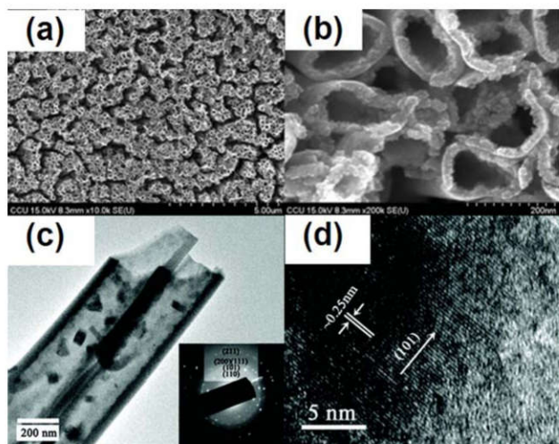
Fig. 5 (a, b) SEM images of a hydrous RuO 2 nanotube arrayed electrode, (c) TEM image and (d) HRTEM image of hydrous RuO 2 nanotubes annealed in air at 200 °C for 2 h. The inset of electron diffraction pattern shows diffraction rings of polycrystalline RuO 2 in the rutile form. Reproduced with permission from ref. 46. Copyright 2006 American Chemical Society.
